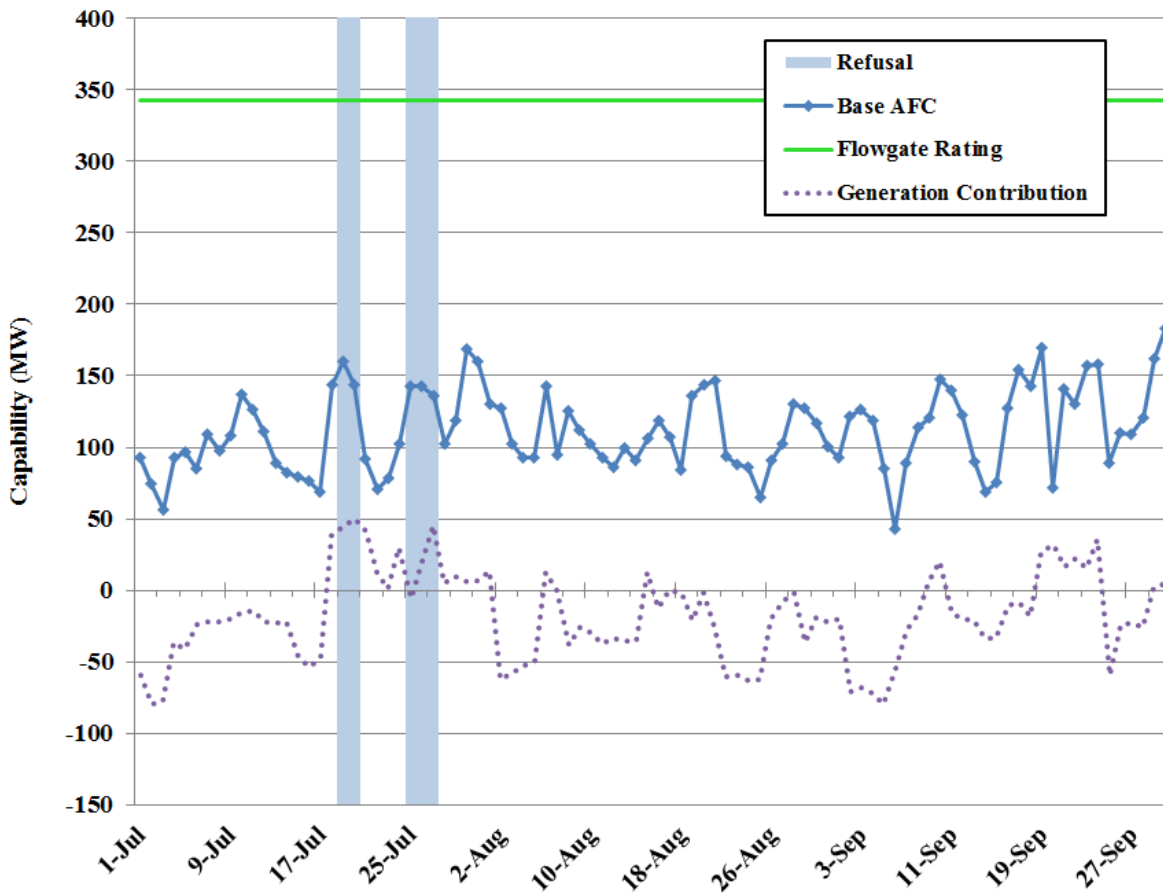
Figure 11: Base AFC –Allen 230/100 kV Transformer (DUK) July 2016 – September 2016
