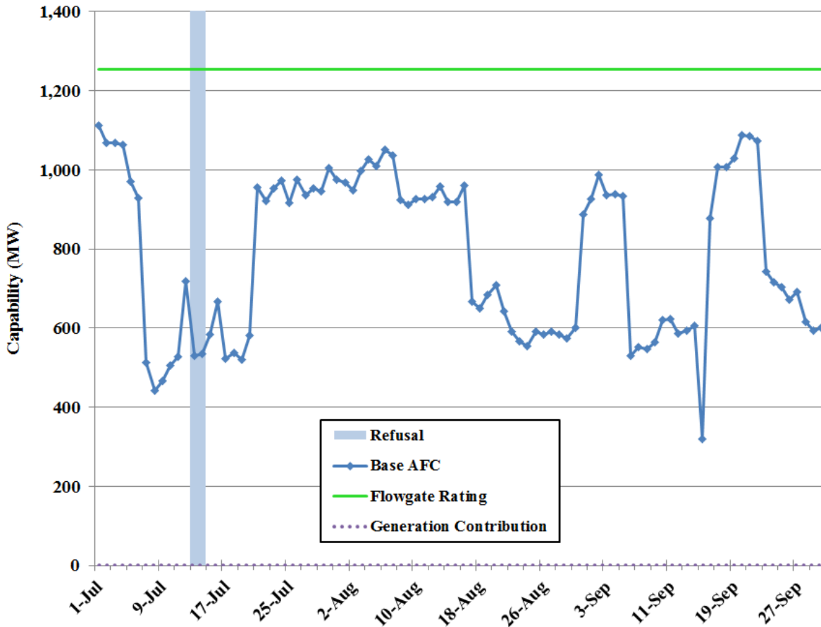
Figure 12: Base AFC – Bull Run 500/161 kV Transformer (TVA) July 2016 – September 2016
