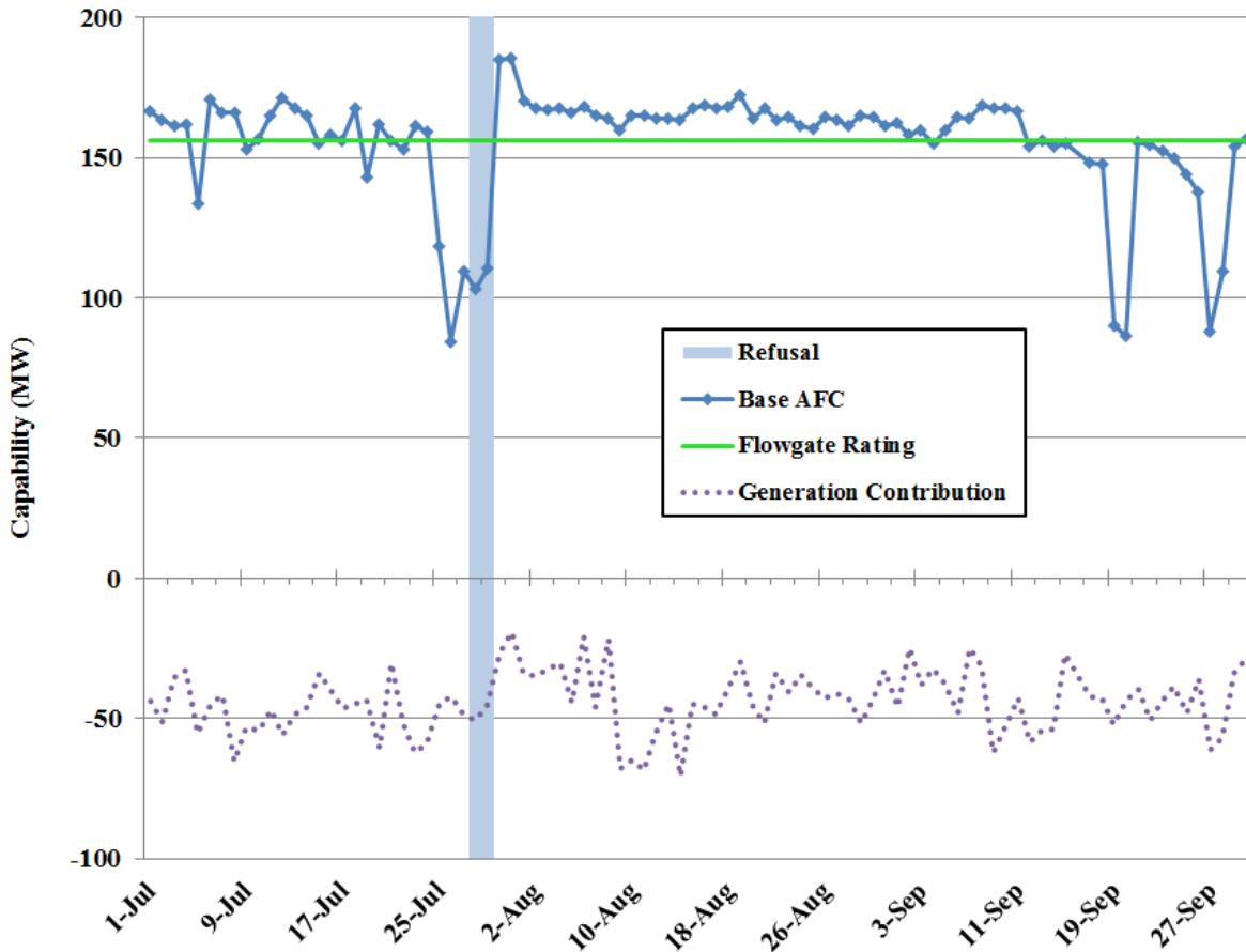
Figure 10: Base AFC – Badin to Albemarle 100 kV (DUK) July 2016 – September 2016
