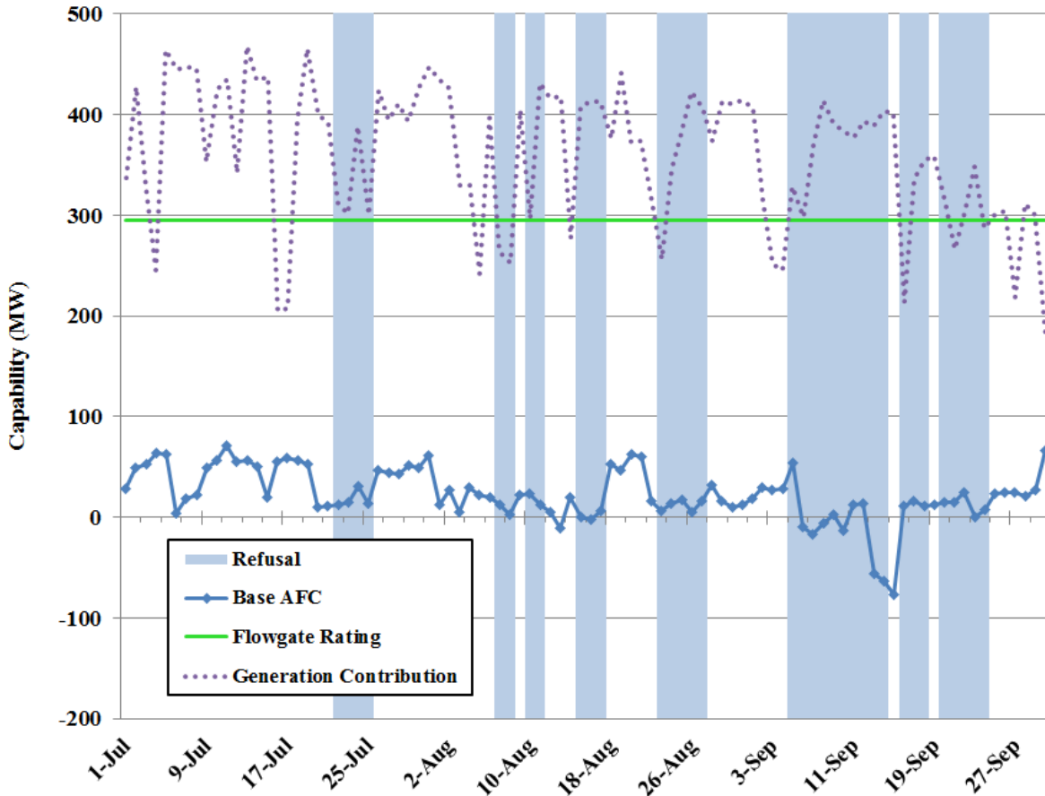
Figure 9: Base AFC – Glen Raven to Burlington 100 kV (DUK) July 2016 – September 2016
