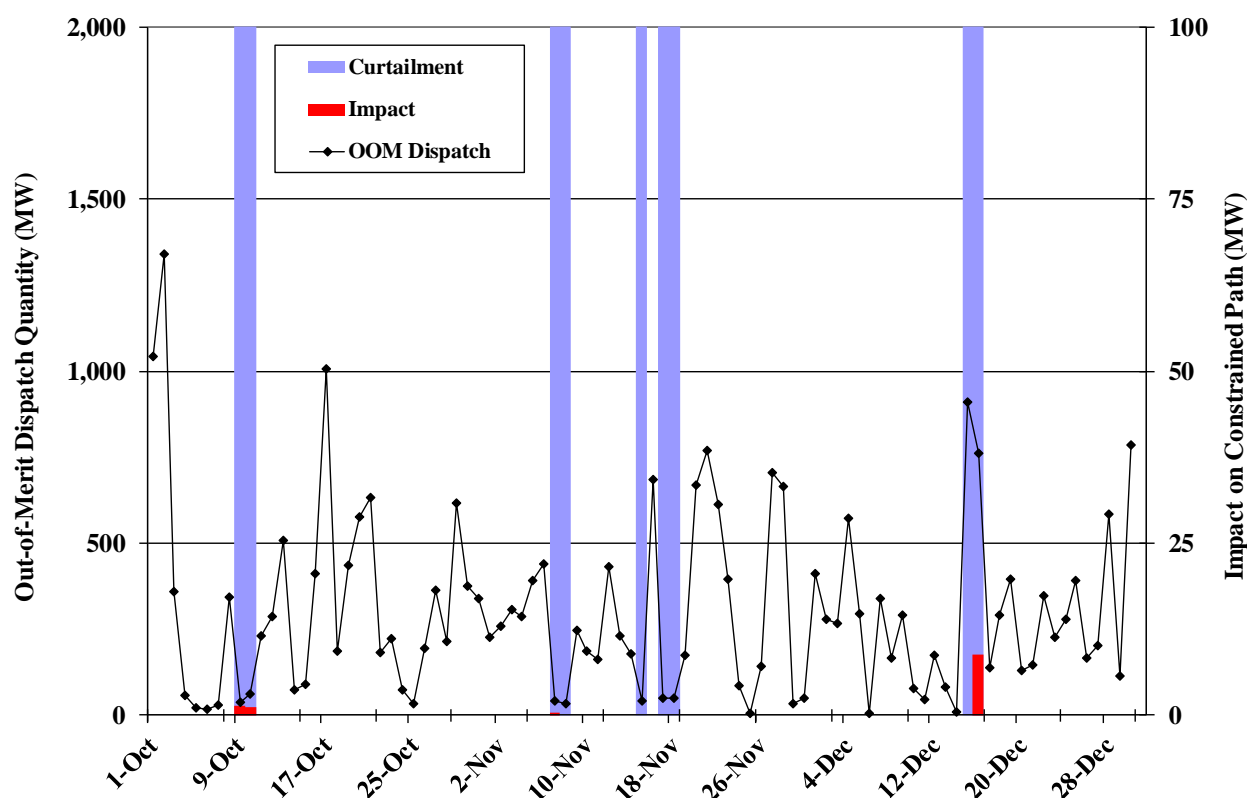
Figure 15: Out-of-Merit Dispatch and Congestion Events October 2016 – December 2016
