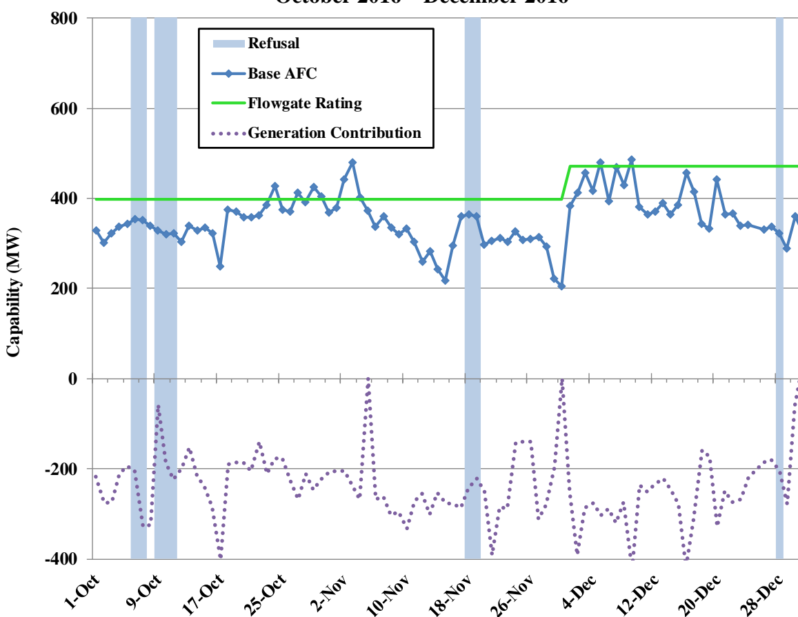
Figure 12: Base AFC – Oakboro to Ansonville 230kV (CPL) October 2016 – December 2016
