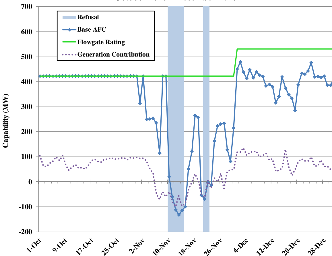
Figure 10: Base AFC – Riverview to Peach Valley 230 kV (DUK) October 2016 – December 2016
