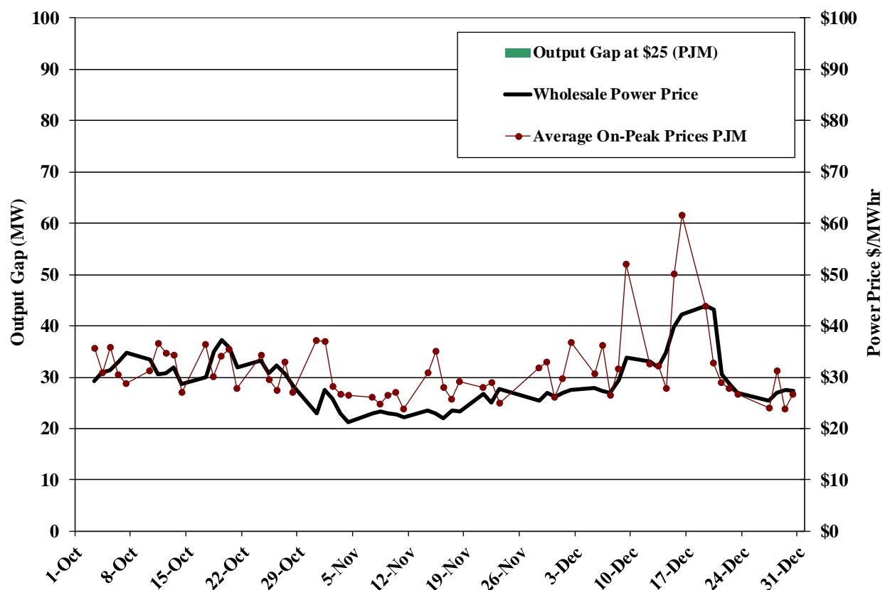
Figure 16: Output Gap October 2016 – December 2016
