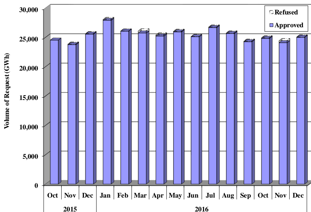
Figure 4: Disposition of Requests for Transmission Service on the Duke System October 2016 – December 2016
