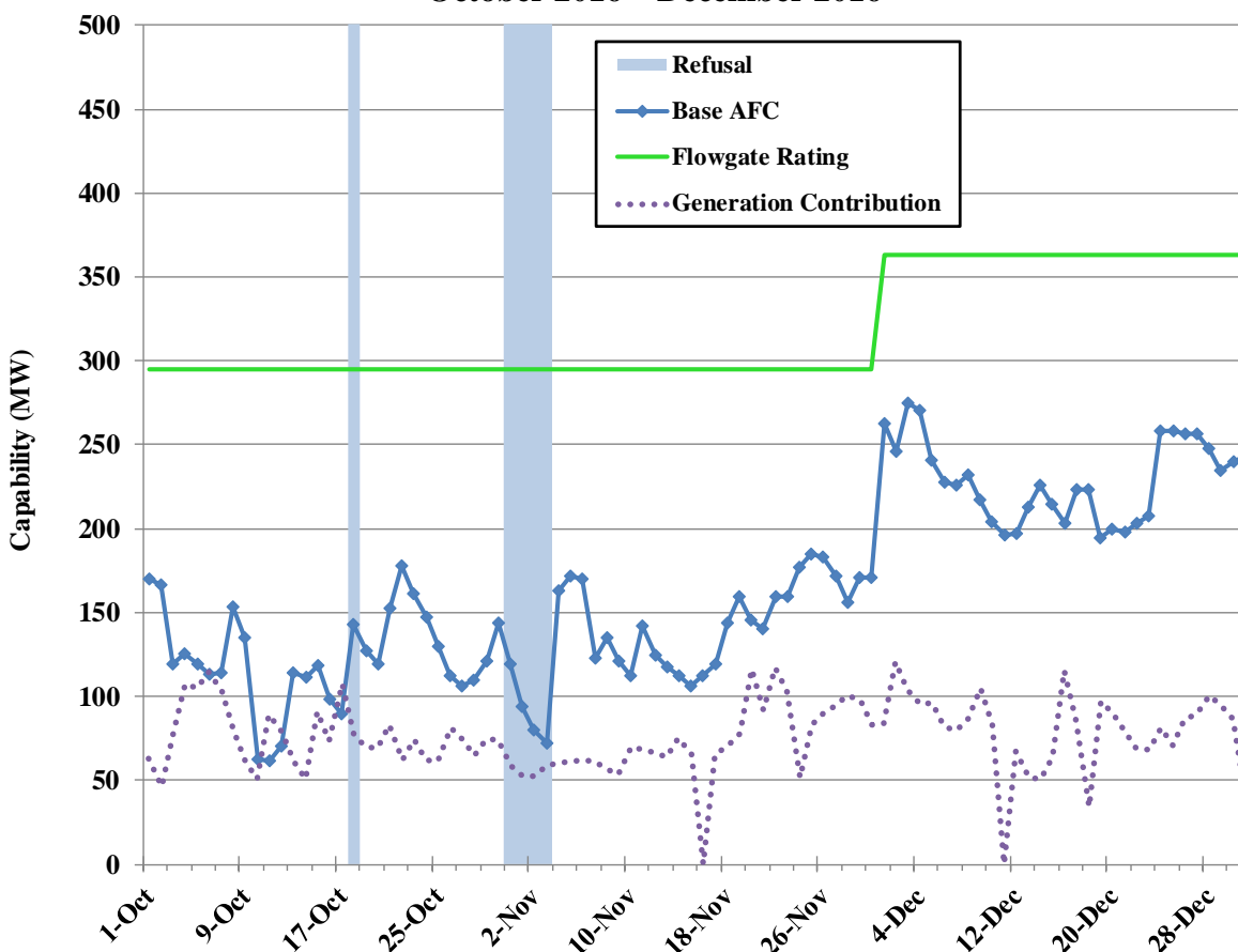
Figure 9: Base AFC – Glen Raven to Burlington 100 kV (DUK) October 2016 – December 2016
