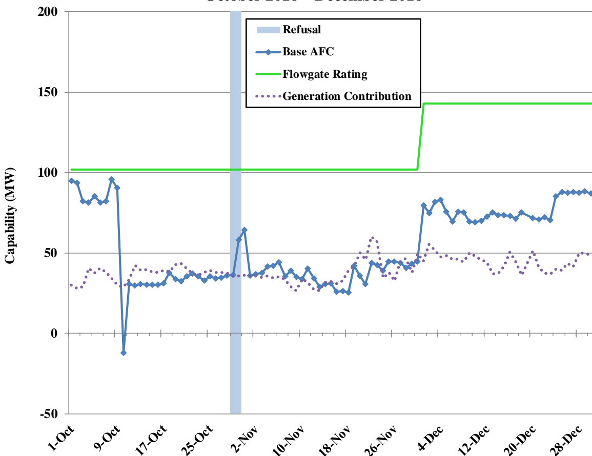
Figure 11: Base AFC –Madison to Unifi Tap 100 kV (DUK) October 2016 – December 2016
