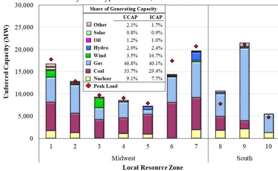
Figure A116: Distribution of Existing Generating Capacity By Fuel Type and Zone, December 2021
