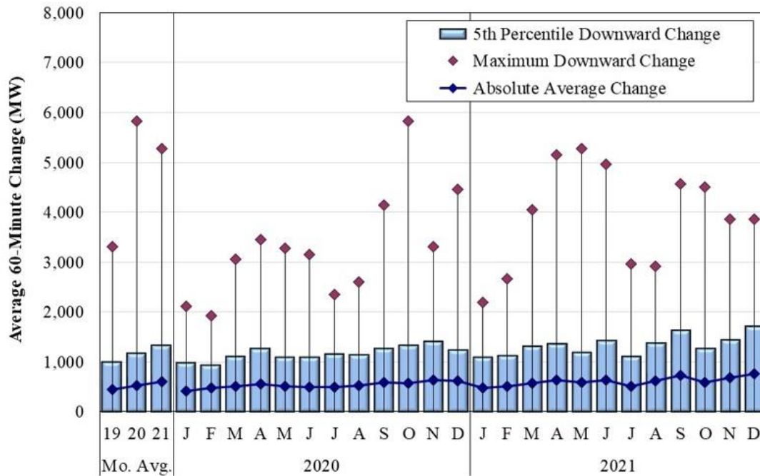
Figure A75: Wind Generation Volatility 2020–2021
