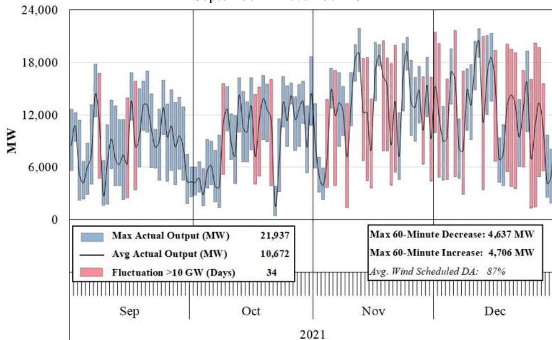
Figure A15: Daily Range of Wind Generation Output September – December 2021
