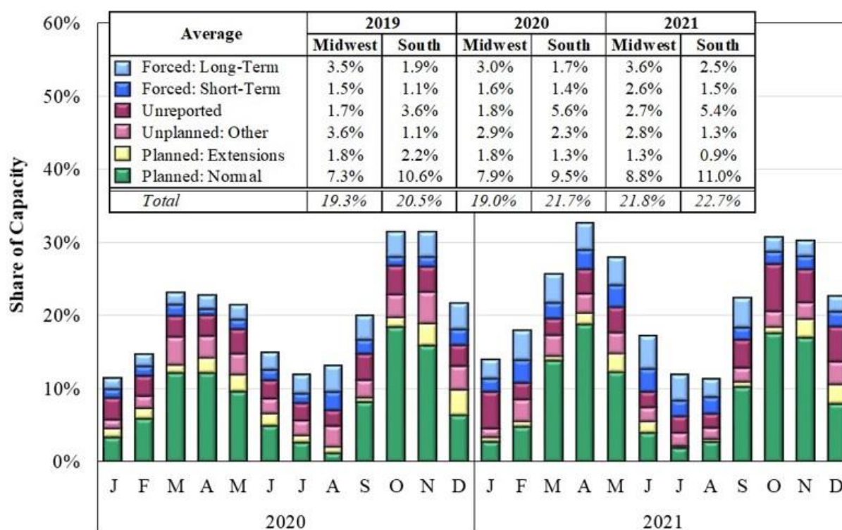
Figure A77: Generator Outage Rates 2019–2021
