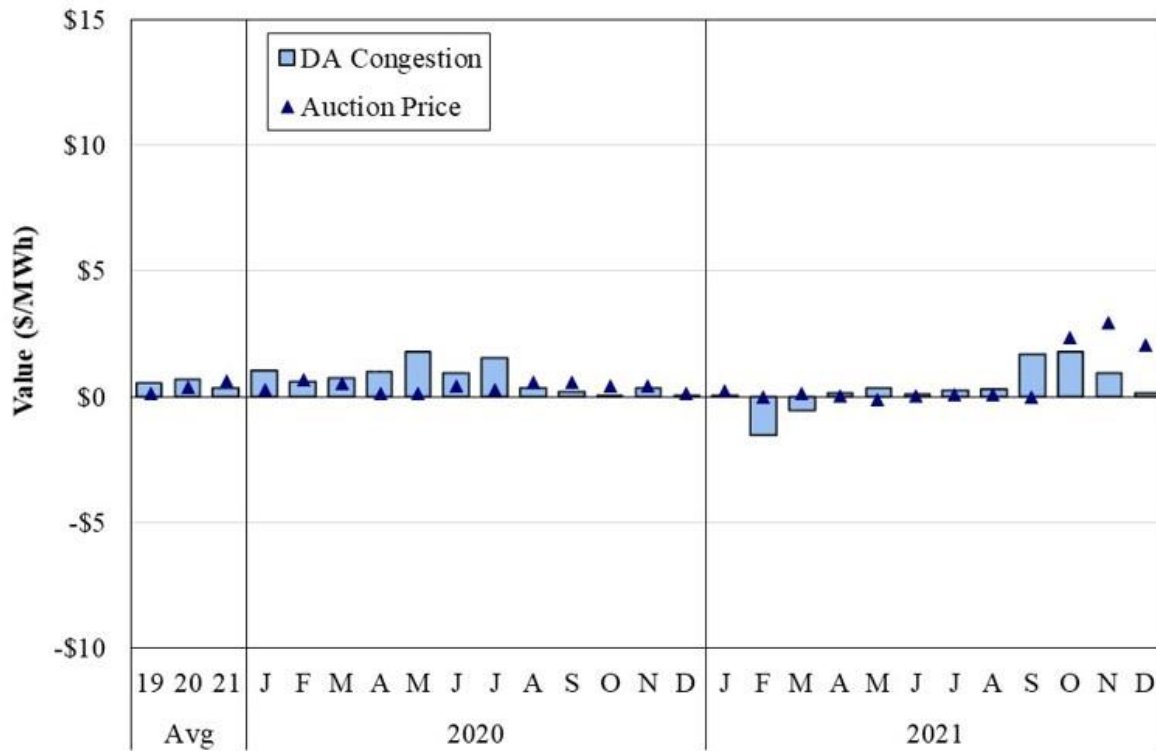
Figure A105: Comparison of FTR Auction Prices and Congestion Value Michigan Hub, 2020–2021: Off-Peak Hours
