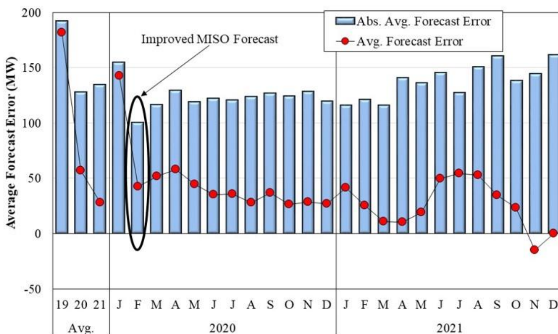
Figure A74: Generation Wind Over-Forecasting Levels 2020–2021
