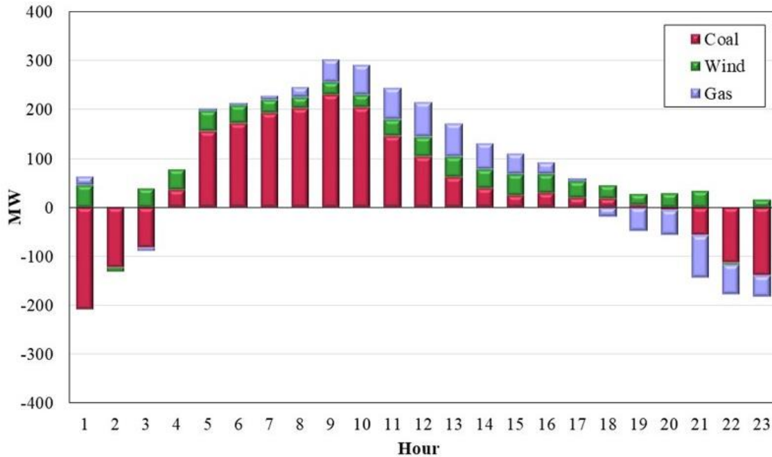
Figure A68: 60-Minute Deviation by Fuel and Hour Summer 2021
