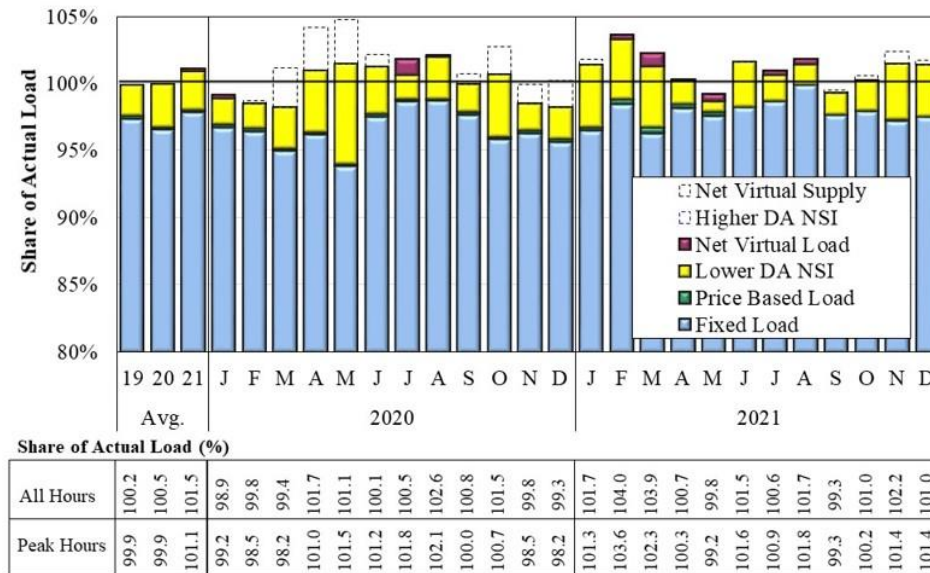
Figure A38: MISO South Day-Ahead Scheduled Versus Actual Loads 2020–2021, Daily Peak Hour
