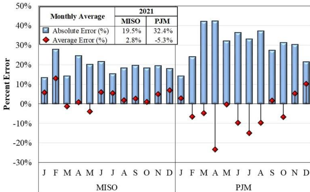
Figure A130: MISO and PJM CTS Forecast Errors 2021
