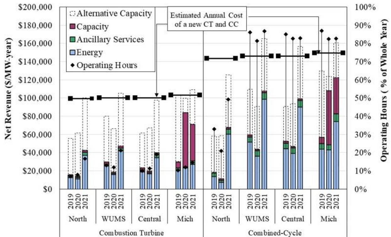
Figure A119: Net Revenue Analysis Midwest Region, 2019–2021
