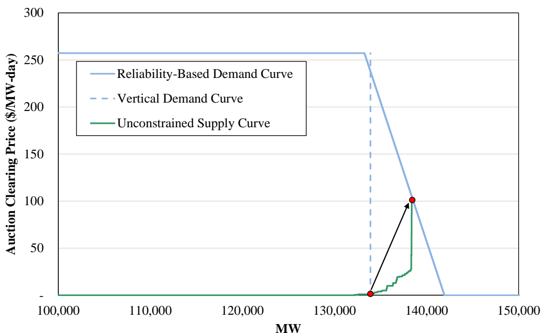
Figure A25: Supply and Demand in 2021/2022 PRA
