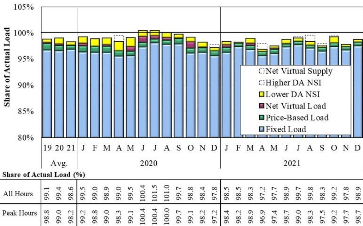
Figure A36: Day-Ahead Scheduled Versus Actual Loads 2020–2021, Daily Peak Hour
