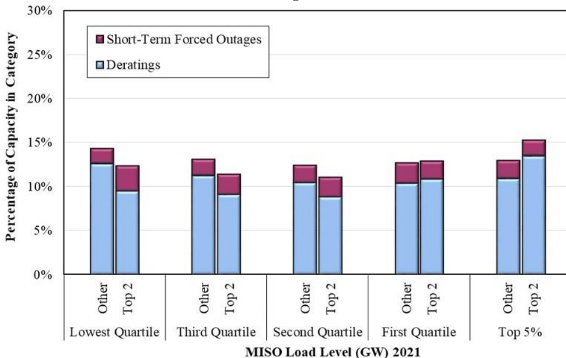
Figure A151: Real-Time Deratings and Forced Outages Central Region, 2021
