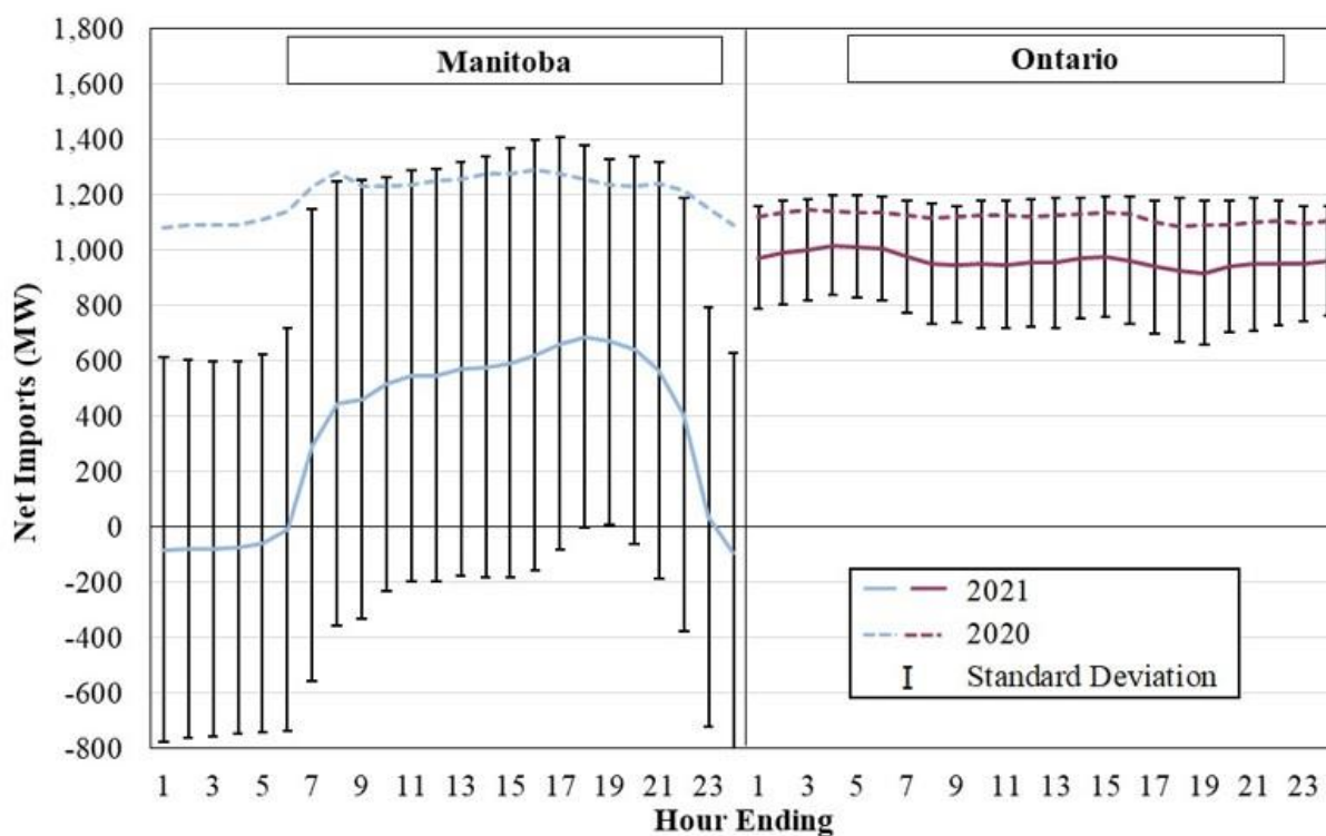
Figure A128: Average Hourly Real-Time Net Imports from Canada 2020–2021
