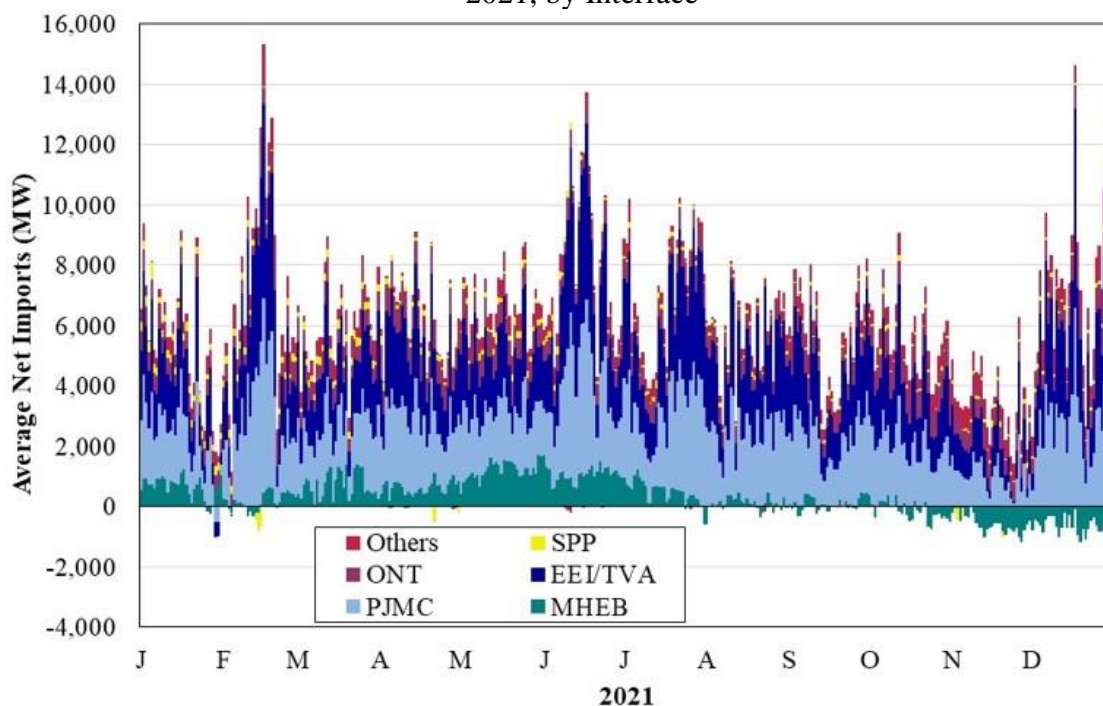
Figure A125: Average Hourly Day-Ahead Net Imports 2021, by Interface
