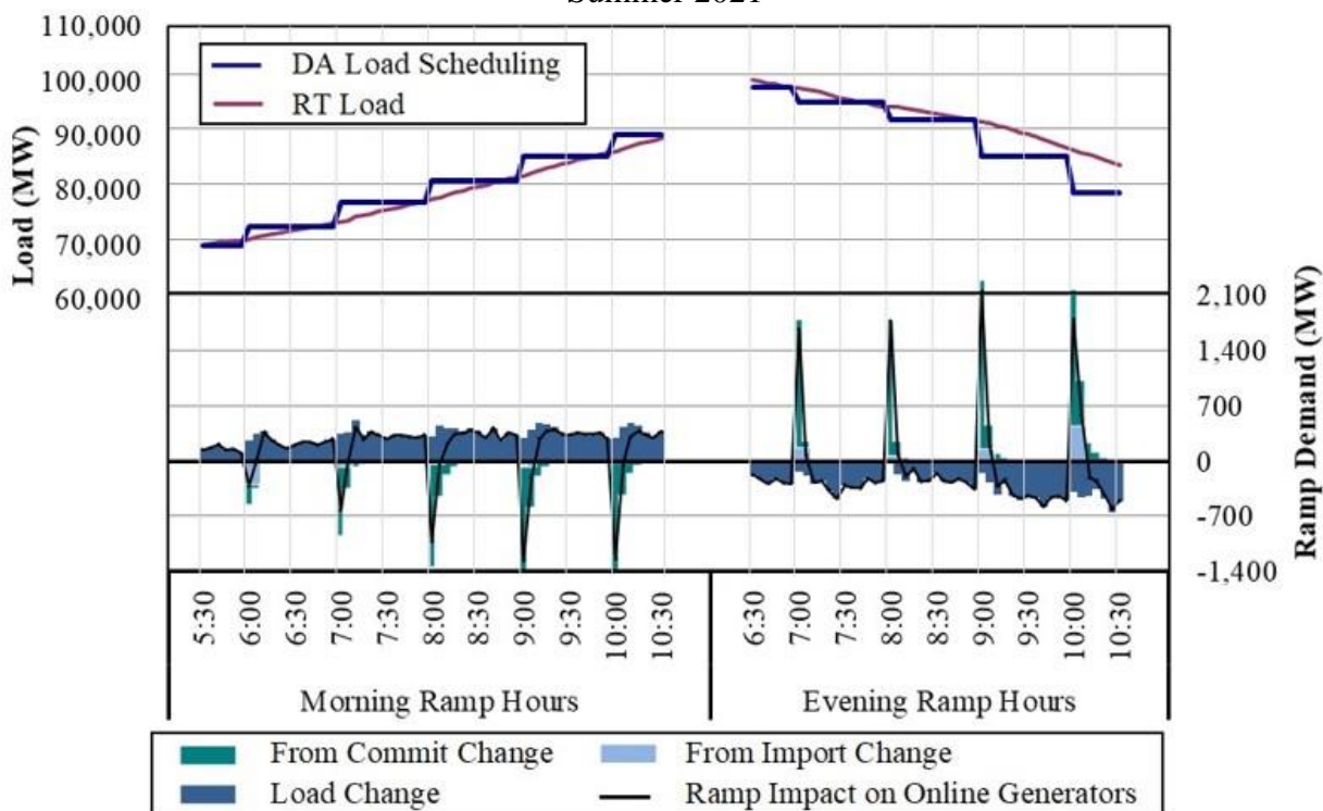
Figure A40: Ramp Demand Impact of Hourly Day-Ahead Market Summer 2021
