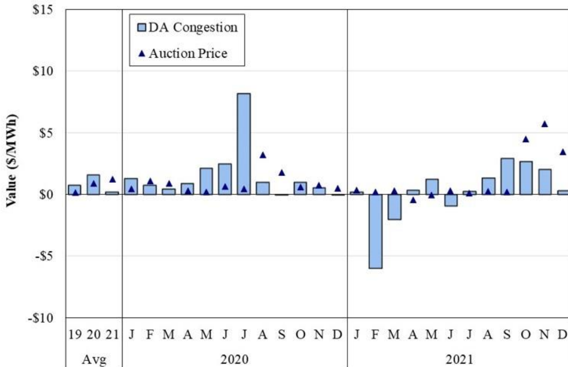
Figure A106: Comparison of FTR Auction Prices and Congestion Value Michigan Hub, 2020–2021: Peak Hours
