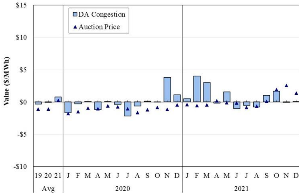
Figure A109: Comparison of FTR Auction Prices and Congestion Value Arkansas Hub, 2020–2021: Off-Peak Hours
