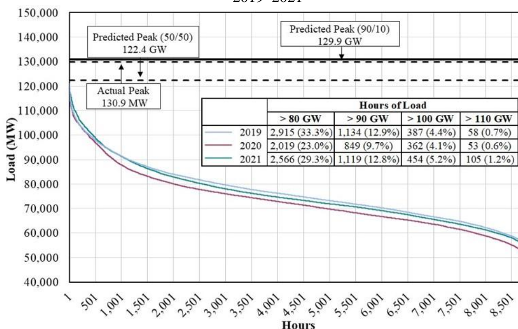
Figure A7: Load Duration Curves and 2021 Peak Load 2019–2021
